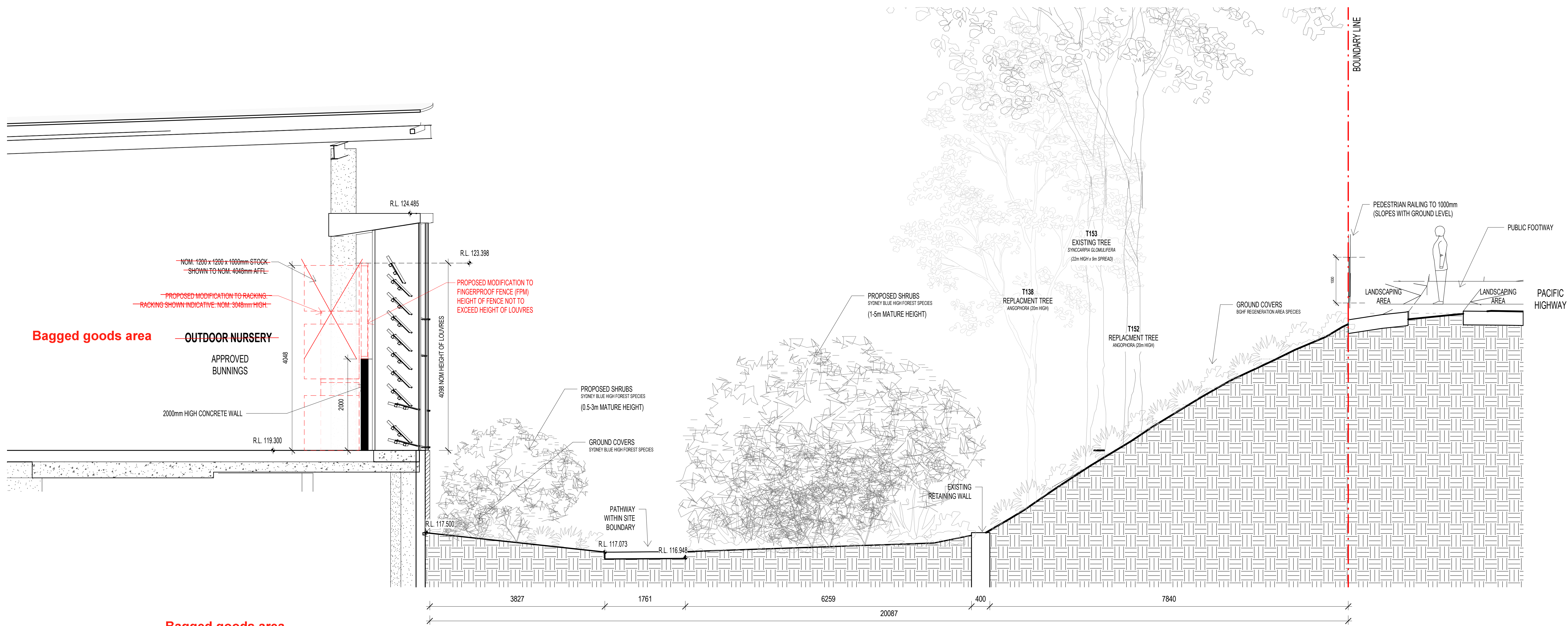
1 SKETCH SECTION THROUGH NURSERY (EXTENDED) 1:40@A0
